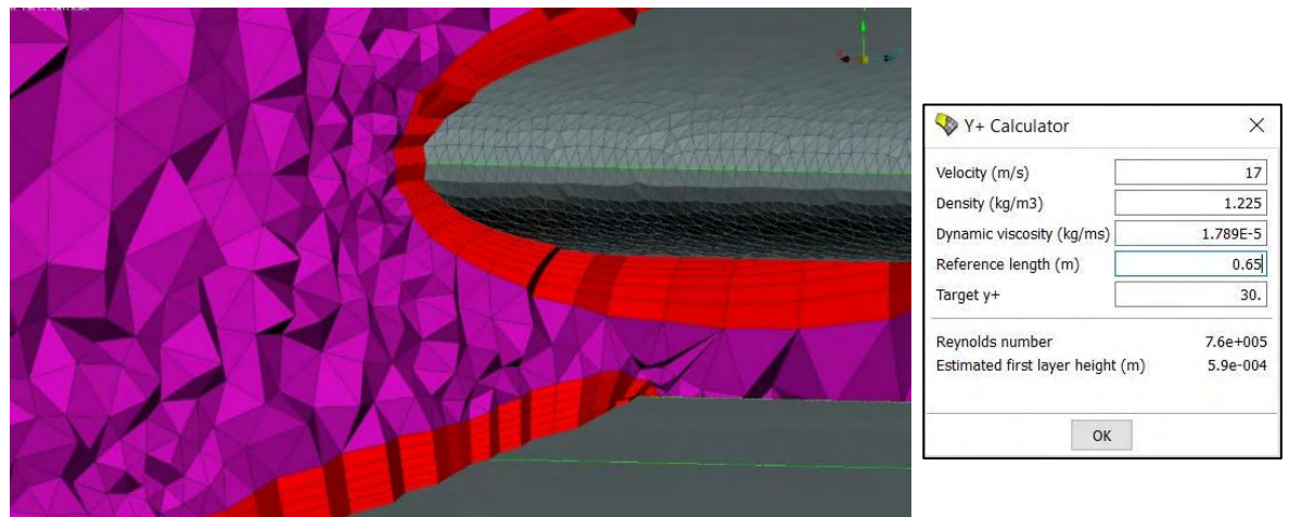
Figure 68: Layers created for front wing model
